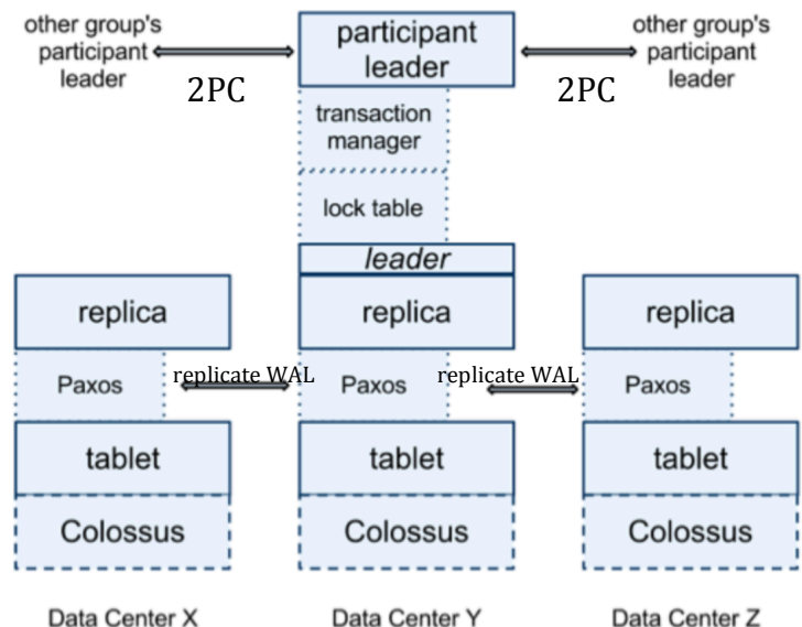
Figure 1. Spanner Architecture.
