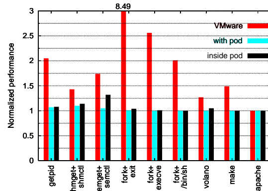
Figure 1: Virtualization cost
